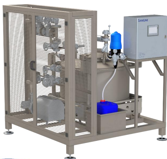
SaniLine 3: Sanitation in line with heating and tank
